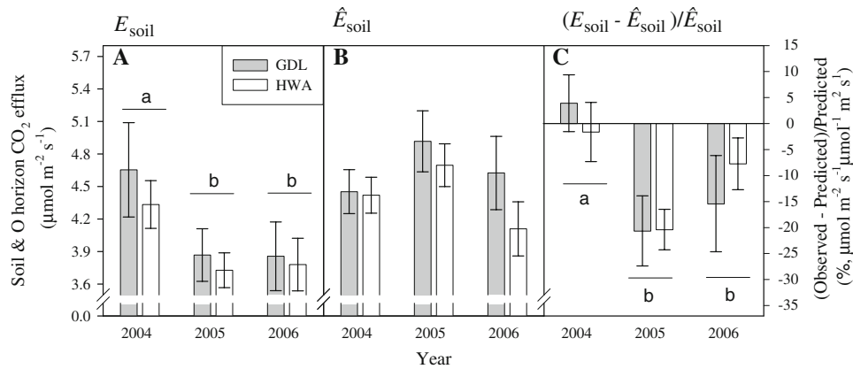
Figure 5. Observed mean soil CO 2 efflux ( E_{soil} ) from soil plus O horizon from the girdled (GDL) and HWA treatments ( A ). Predicted responses ( \hat{E}_{soil} ) in ( B ), and the deviance from predicted values ( C ). Bars denote standard error. Different letters in ( A ) and ( C ) denote significant differences among years. Girdling occurred in July 2004. HWA infestation was observed in December 2004
