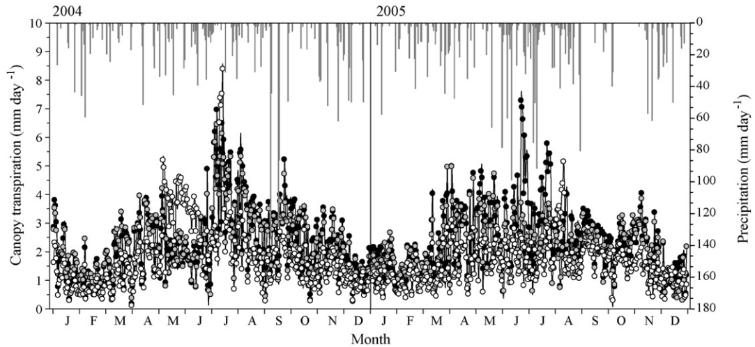
Fig. 2. Mean daily precipitation (grey bars) and canopy transpiration in experimental plots G1 (black circles), G2 (grey circles), and G3 (white circles) during 2004 and 2005. Plot estimates of annual E_t for 2004 and 2005 were 840.7 and 864.5 mm year -1 (G1), 818.6 and 746.3 mm year -1 (G2), 650.5 and 576.8 mm year -1 (G3).
